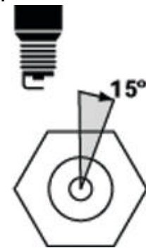
Spark Plug with Tapered Seat
